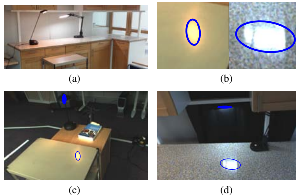
Figure 1: We observe that specularities have a conic shape on planar surfaces. We approximate them by projecting a fixed quadric which includes light and material properties. This figure presents quadric reconstruction examples (blue quadrics) for two light types (light bulb (c) and fluorescent lamp (d)) and two materials (steel table (c) and a plastic kitchen counter (d)). The lights sources along with the steel table and the plastic kitchen counter can be seen in (a). Once reconstructed, our virtual quadric model allows the prediction of future specular reflections by simple perspective projection (blue conics). (b) shows the specularity prediction close-up in the respective sequences.
