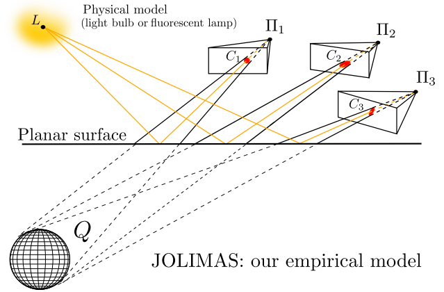
Figure 2: JOLIMAS illustration, showing the link between photometry (light and surface material) and multiple view geometry (our empirical model). The light source L which could be either a light bulb or a fluorescent lamp is creating specularities (the red conics) in the different viewpoints \Pi_1 , \Pi_2 and \Pi_3 . From multiple viewpoints, a quadric Q is reconstructed from specular reflections of conic shape in the images ( C_1 , C_2 and C_3 ). We then use the quadric Q projected onto the planar surface to predict specularities in new viewpoints.
