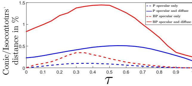
Figure 4: Empirical validation from simulated data. Our hypothesis of conic shaped specularities is tested on the Phong (P) and the Blinn-Phong (BP) illumination models for different values of intensity \tau \in [0, 1] . This hypothesis is tested for the specular term alone and for the combination of the specular and diffuse terms. For each value of \tau , with a step of 0.05 between each value, we run 1000 scenarios of different light source and camera poses. The error is computed using the distance from Sturm et al. [35] between the fitted conic and the isocontours for each scenario.
