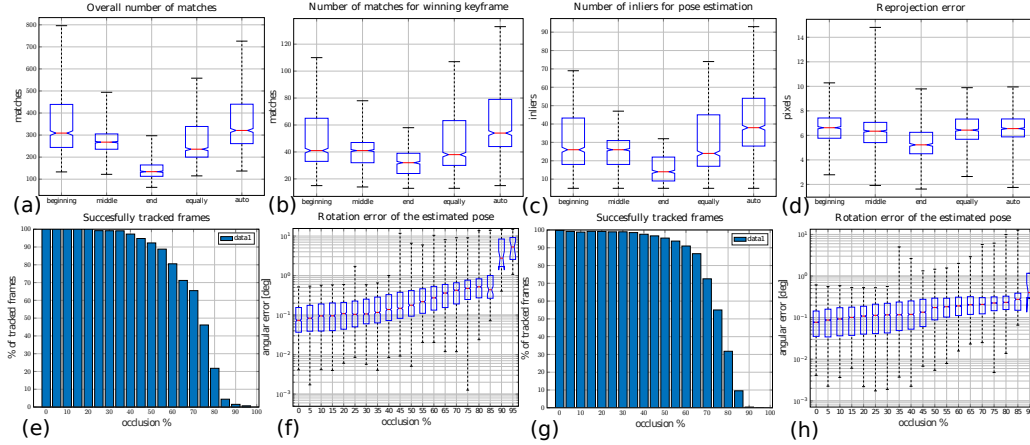
Fig. 11: (a,b,c,d) Tracking statistics (number of matches, inliers, and pose errors) for each keyframe sampling method.(e,f,g,h) From left to right, histogram of successfully tracked frames and rotation error of estimated pose, for both experiments.
