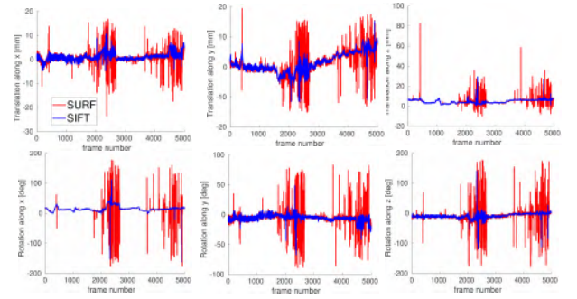
Fig. 5: Comparing SURF and SIFT on 5000 video frames.
